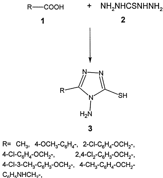
SCHEME 2 Synthesis of 4-amino-3-substituted-5-mercapto-1,2,4-triazoles ( 3 ).
